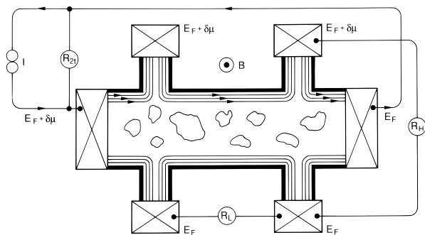
FIG. 79 Measurement configuration for the two-terminal resistance R_{2t} , the four-terminal Hall resistance R_H , and the longitudinal resistance R_L . The edge channels at the Fermi level are indicated; arrows point in the direction of motion of edge channels filled by the source contact at chemical potential E_F + \delta\mu . The current is equipartitioned among the edge channels at the upper edge, corresponding to the case of local equilibrium.
