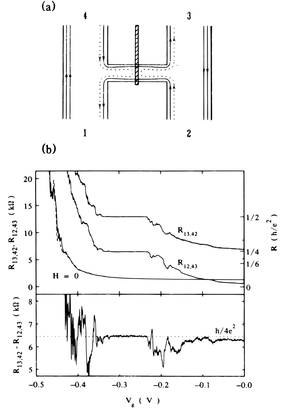
FIG. 85 (a) Schematic view of a 2\text{-}\mu\text{m} -wide channel containing a potential barrier imposed by a 0.1\text{-}\mu\text{m} -long gate. (b) Top: diagonal resistance R_{13,42} \equiv R_D^+ and longitudinal resistance R_{12,43} \equiv R_L as a function of gate voltage in a strong magnetic field ( B = 5.2 T), showing a quantized plateau in agreement with Eqs. (4.14) and (4.12), respectively. For comparison also the two zero-field traces are shown, which are almost identical. Bottom: Difference R_D^+ - R_L = R_H at 5.2 T. A normal quantum Hall plateau is found, with oscillatory structure superimposed in gate voltage regions where R_D^+ and R_L are not quantized. Taken from S. Washburn et al., Phys. Rev. Lett. 61 , 2801 (1988).
