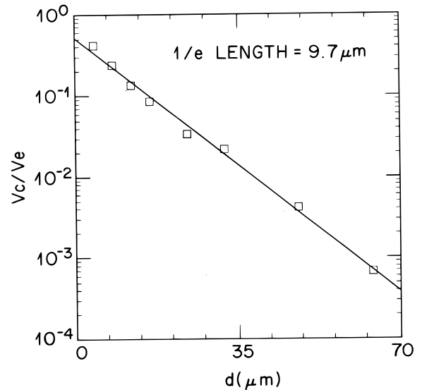
FIG. 58 Exponential decay of the oscillation amplitude of the collector voltage (normalized by the injector voltage) as a function of injector-collector separation d (denoted by L in the text). Taken from J. Spector et al., Surf. Sci. 228 , 283 (1990).
