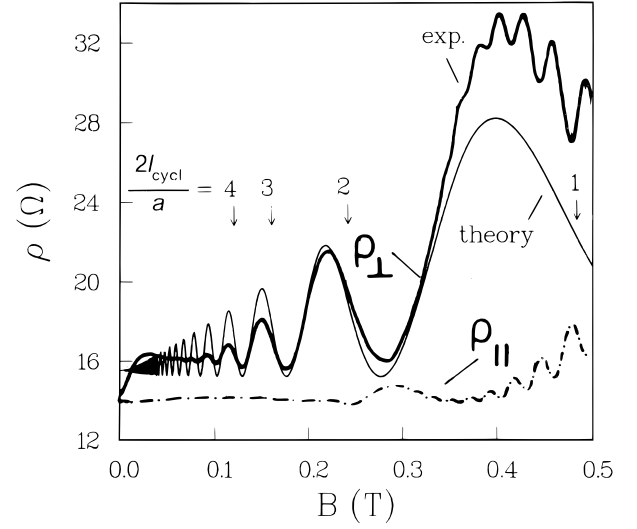
FIG. 37 Solid curves: Magnetic field dependence of the resistivity \rho_{\perp} for current flowing perpendicular to a potential grating. The experimental curve is the measurement of Weiss et al. 255 the theoretical curve follows from the guiding-center-drift resonance. Note the phase shift of the oscillations, indicated by the arrows at integer 2l_{\text{cycl}}/a . The potential grating has periodicity a = 382 nm and is modeled by a sinusoidal potential with root-mean-square amplitude of \epsilon = 1.5\% of the Fermi energy; The mean free path in the 2DEG is 12 \mu\text{m} , much larger than a . The dash-dotted curve is the experimental resistivity \rho_{\parallel} for current flowing parallel to the potential grating, as measured by Weiss et al. Taken from C. W. J. Beenakker, Phys. Rev. Lett. 62 , 2020 (1989).
