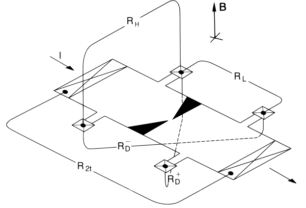
FIG. 82 Perspective view of a six-terminal Hall bar containing a point contact, showing the various two- and four-terminal resistances mentioned in the text. Taken from H. van Houten et al., in Ref. 9 .
