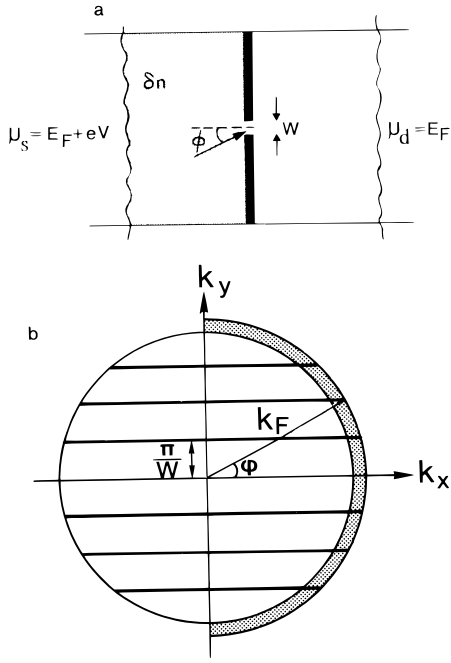
FIG. 45 (a) Classical ballistic transport through a point contact induced by a concentration difference \delta n , or electrochemical potential difference eV , between source (s) and drain (d). (b) The net current through a quantum point contact is carried by the shaded region in k -space. In a narrow channel the allowed states lie on the horizontal lines, which correspond to quantized values for k_y = \pm n\pi/W , and continuous values for k_x . The formation of these 1D subbands gives rise to a quantized conductance. Taken from H. van Houten et al., in “Physics and Technology of Submicron Structures” (H. Heinrich, G. Bauer, and F. Kuchar, eds.). Springer, Berlin, 1988; and in “Nanostructure Physics and Fabrication” (M. Reed and W. P. Kirk, eds.). Academic, New York, 1989.
