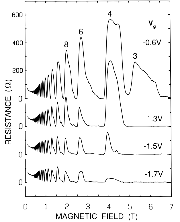
FIG. 93 Measurement of the anomalous Shubnikov-De Haas oscillations in the geometry of Fig. 92. The plotted longitudinal resistance is the voltage drop between contacts p and d divided by the current from s to d. At high magnetic fields the oscillations are increasingly suppressed as the point contact in the voltage probe is pinched off by increasing the negative gate voltage. The number of occupied spin-split Landau levels in the bulk is indicated at several of the Shubnikov-De Haas maxima. Taken from B. J. van Wees et al., Phys. Rev. B 39 , 8066 (1989).
