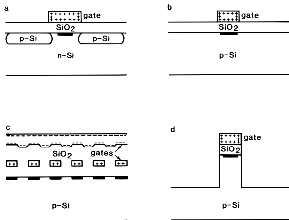
FIG. 2 Schematic cross-sectional views of the lateral pinch-off technique used to define a narrow electron accumulation layer (a), and of three different methods to define a narrow electron inversion layer in Si MOSFET's (b-d). Positive (+) and negative (-) charges on the gate electrodes are indicated. The location of the 2DEG is shown in black.
