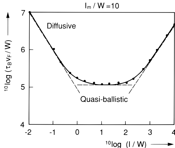
FIG. 18 Phase relaxation time \tau_B in a channel with specular boundary scattering, as a function of the elastic mean free path l . The plot has been obtained by a numerical simulation of the phase relaxation process for a magnetic field such that l_m = 10W . The dashed lines are analytic formulas valid in the three asymptotic regimes (see Table II). Taken from C. W. J. Beenakker and H. van Houten, Phys. Rev. B 38 , 3232 (1988).
