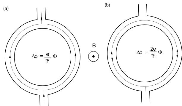
FIG. 25 Illustration of the Aharonov-Bohm effect in a ring geometry. Interfering trajectories responsible for the magnetoconductance oscillations with h/e periodicity in the enclosed flux \Phi are shown (a). (b) The pair of time-reversed trajectories lead to oscillations with h/2e periodicity.
